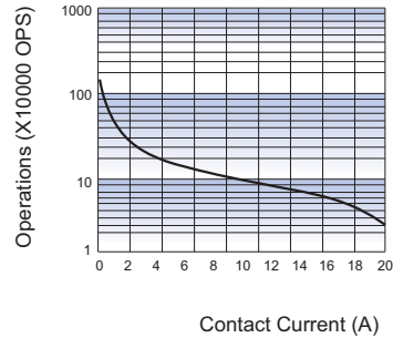
ENDURANCE CURVE
