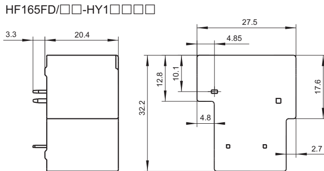
Outline Dimensions
