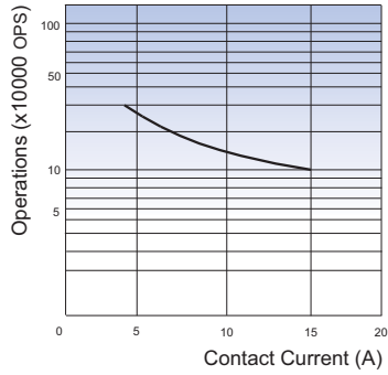
ENDURANCE CURVE
