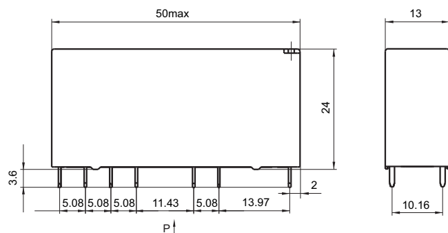
Outline Dimensions
