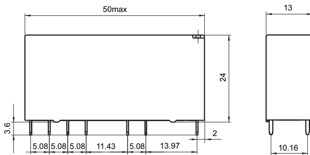
Outline Dimensions
