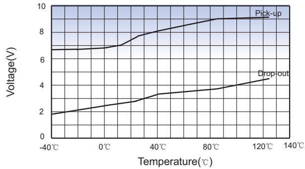
Pick-up Voltage / Drop-out Voltage Curve
