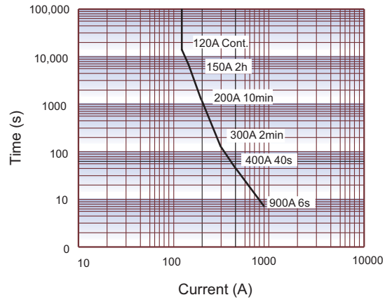
Endurance Capacity Curve
