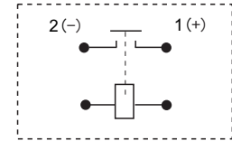
Coil Wiring Diagram
