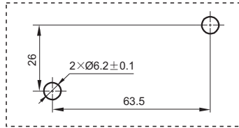
Installation Hole
