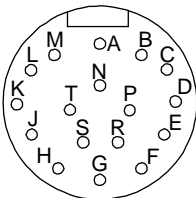
Connector P Encoder connector D/MS3102A20-29P
