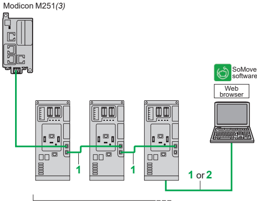
Modicon M251 + ATV340 Ethernet
