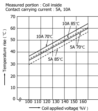
3-2. Coil temperature characteristics (1 Form C)
