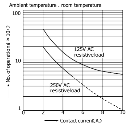
2. Switching life curve (Form A contact)
