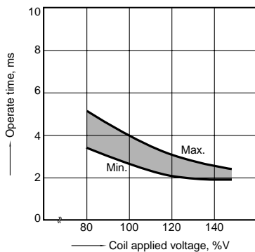
4-(1). Operate time
