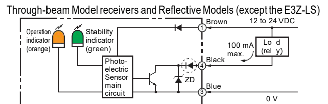
Protection for NPN output models
