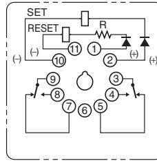
Terminal Arrangement/Internal Connections (Bottom View)
