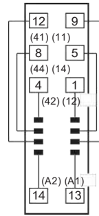
(Top View)
