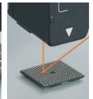
Diffuse reflection
